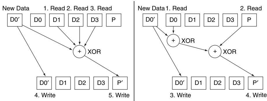
FIGURE 6.13 Small write update on RAID 4. This optimization for small writes reduces the number of disk accesses as well as the number of disks occupied. This figure assumes we have four blocks of data and one block of parity. The naive RAID 4 parity calculation in the left of the figure reads blocks D1, D2, and D3 before adding block D0' to calculate the new parity P'. (In case you were wondering, the new data D0' comes directly from the CPU, so disks are not involved in reading it.) The RAID 4 shortcut on the right reads the old value D0 and compares it to the new value D0' to see which bits will change. You then read the old parity P and then change the corresponding bits to form P'. The logical function exclusive OR does exactly what we want. This example replaces three disk reads (D1, D2, D3) and two disk writes (D0', P') involving all the disks for two disk reads (D0, P) and two disk writes (D0', P'), which involve just two disks. Increasing the size of the parity group increases the savings of the shortcut. RAID 5 uses the same shortcut.
